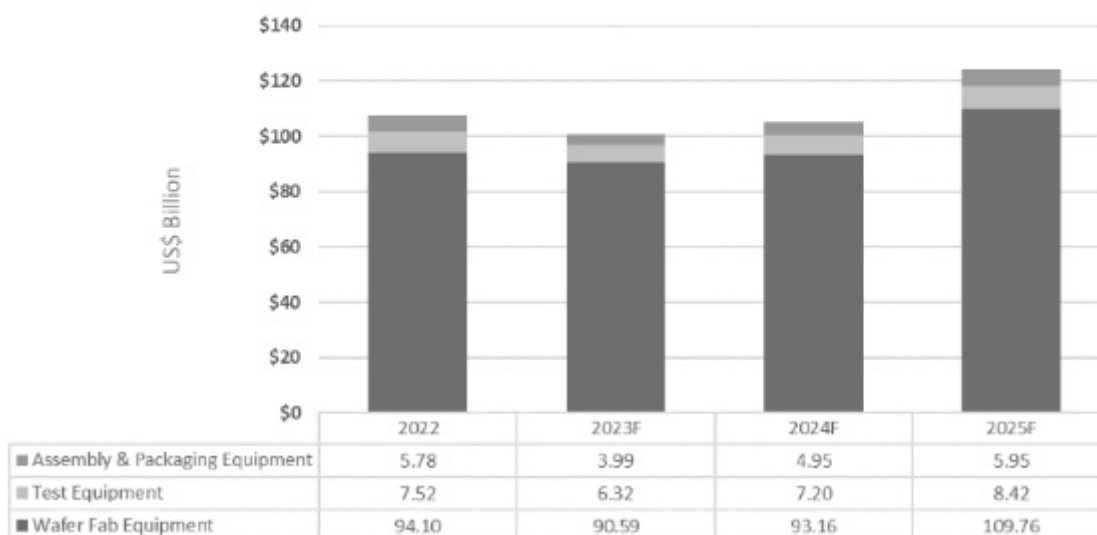
SEMI 2023 Year-End Total Equipment Forecast by Segment (US$ Billion)
