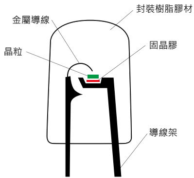
▲ LED 固晶膠
